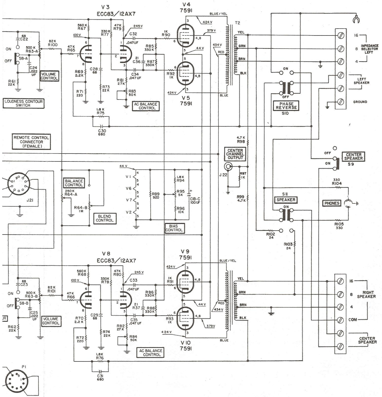
P849 SCHEMATIC AW #1877
